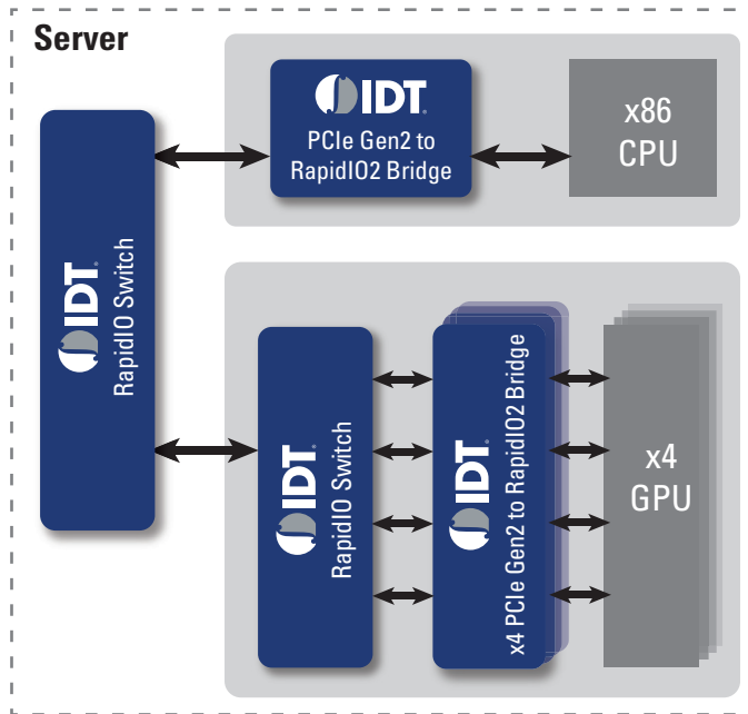
MEC with GPU acceleration: IDT and its partners have demonstrated this system, which scales to 1/2 petaflop per rack.
