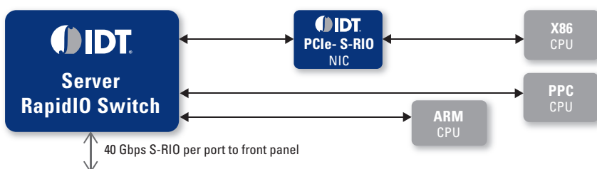
Heterogeneous MEC board block diagram.
